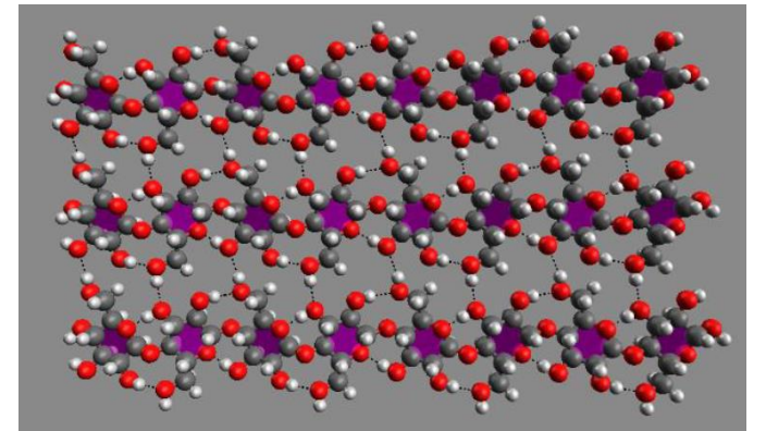
Cellulose structure
